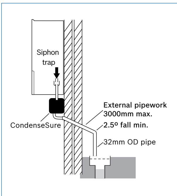
A typical installation using CondenseSure
